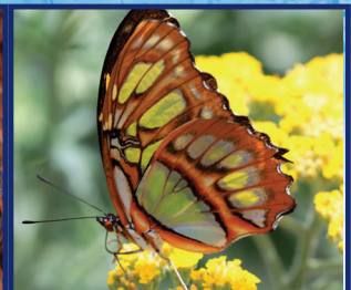
Malachite
