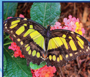
Malachite
